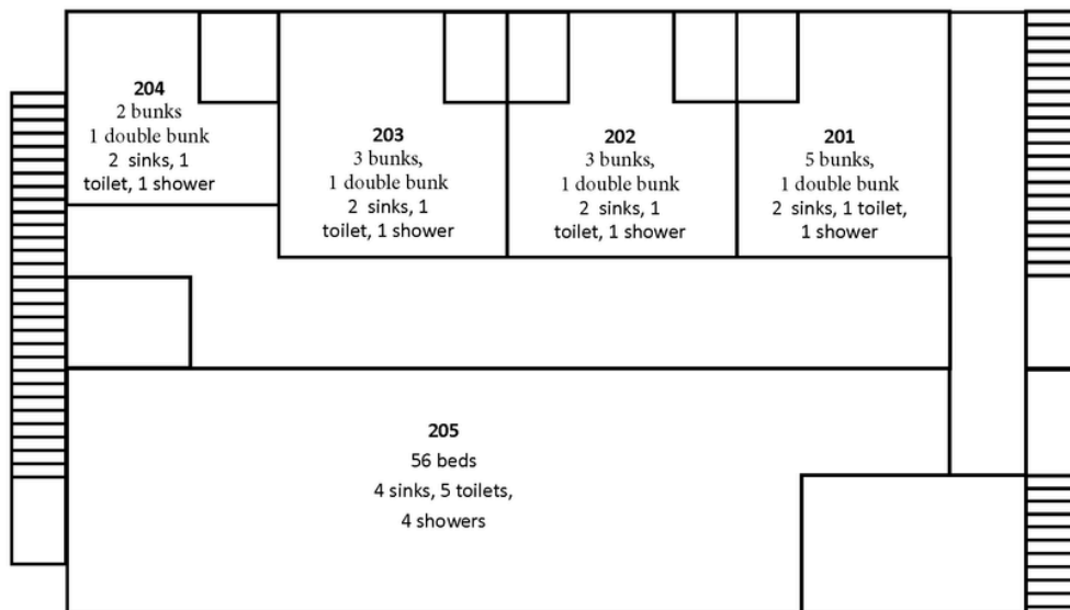
Third Floor Layout
